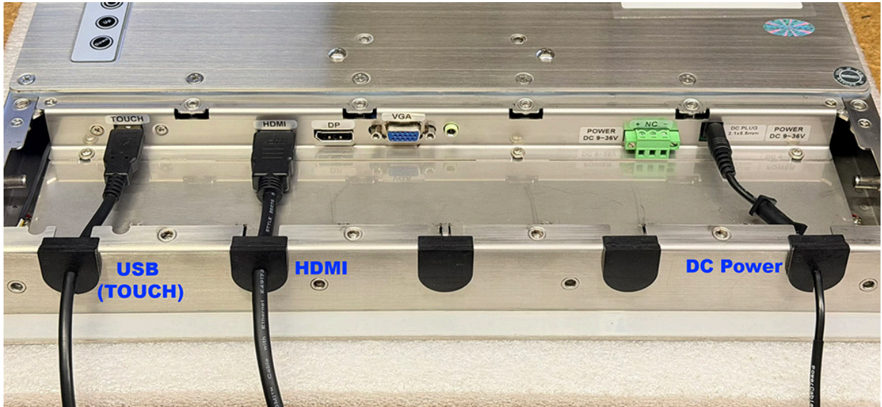
P5. Cables together with Waterproof Rubber Cable Grommets installed into Input Compartment.
